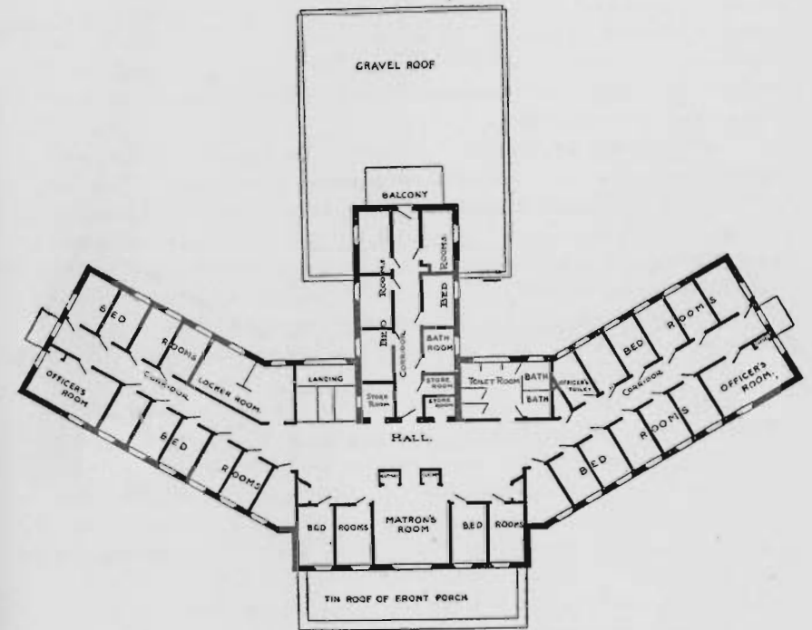
INDIANA GIRLS' SCHOOL, CLERMONT, INDIANA COTTAGE—SECOND-FLOOR PLAN
