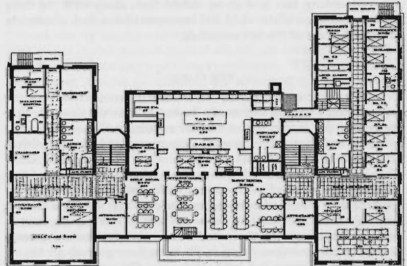
THIRD-FLOOR PLAN MILWAUKEE JUVENILE COURT
