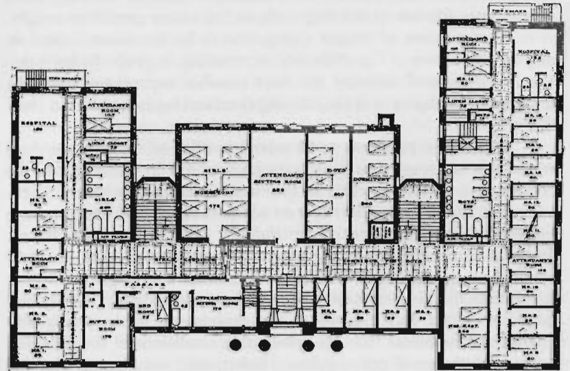
SECOND-FLOOR PLAN
