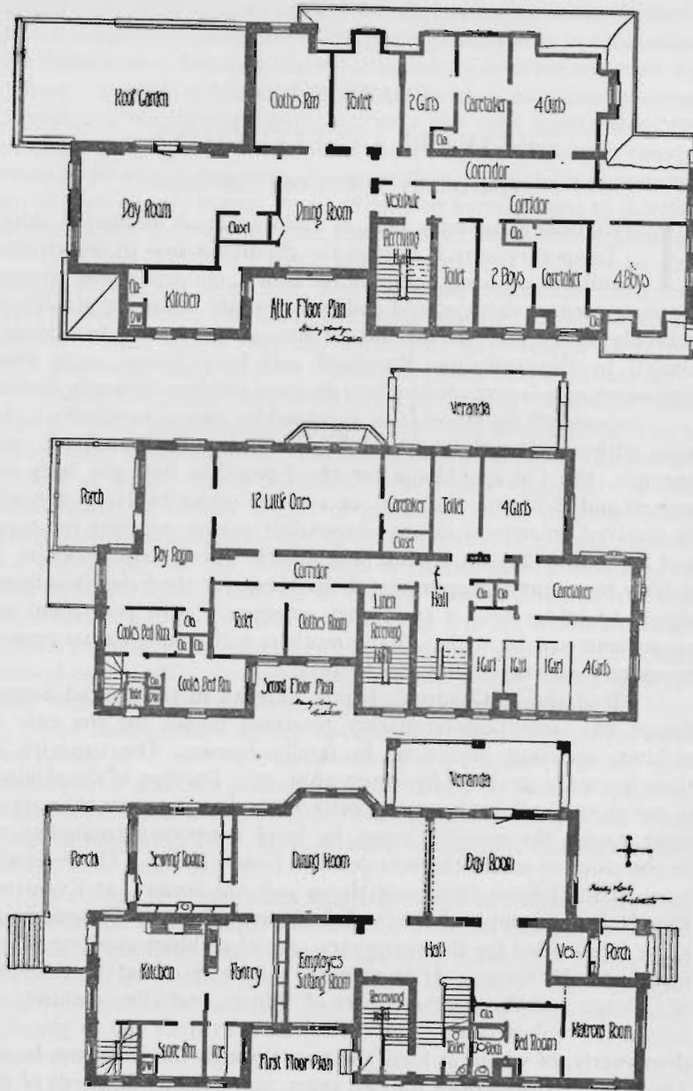
EVANSTON RECEIVING HOME—FLOOR PLANS
