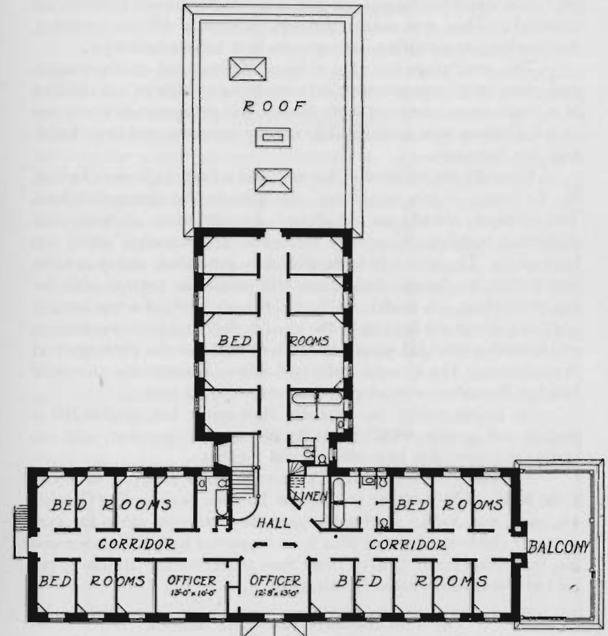
PHILADELPHIA HOUSE OF REFUGE FOR GIRLS, DARLING, PENNSYLVANIA COTTAGE—SECOND-FLOOR PLAN
