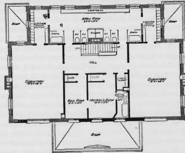
SECOND FLOOR PLAN COTTAGES FOR CHILDREN
